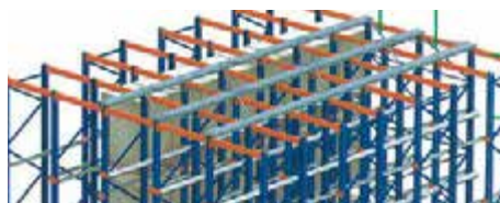
COMPONENTES DRIVE-IN DRIVE-IN COMPONENTS COMPONENTES DRIVE-IN COMPONENTS DRIVE-IN PÁG. 19
